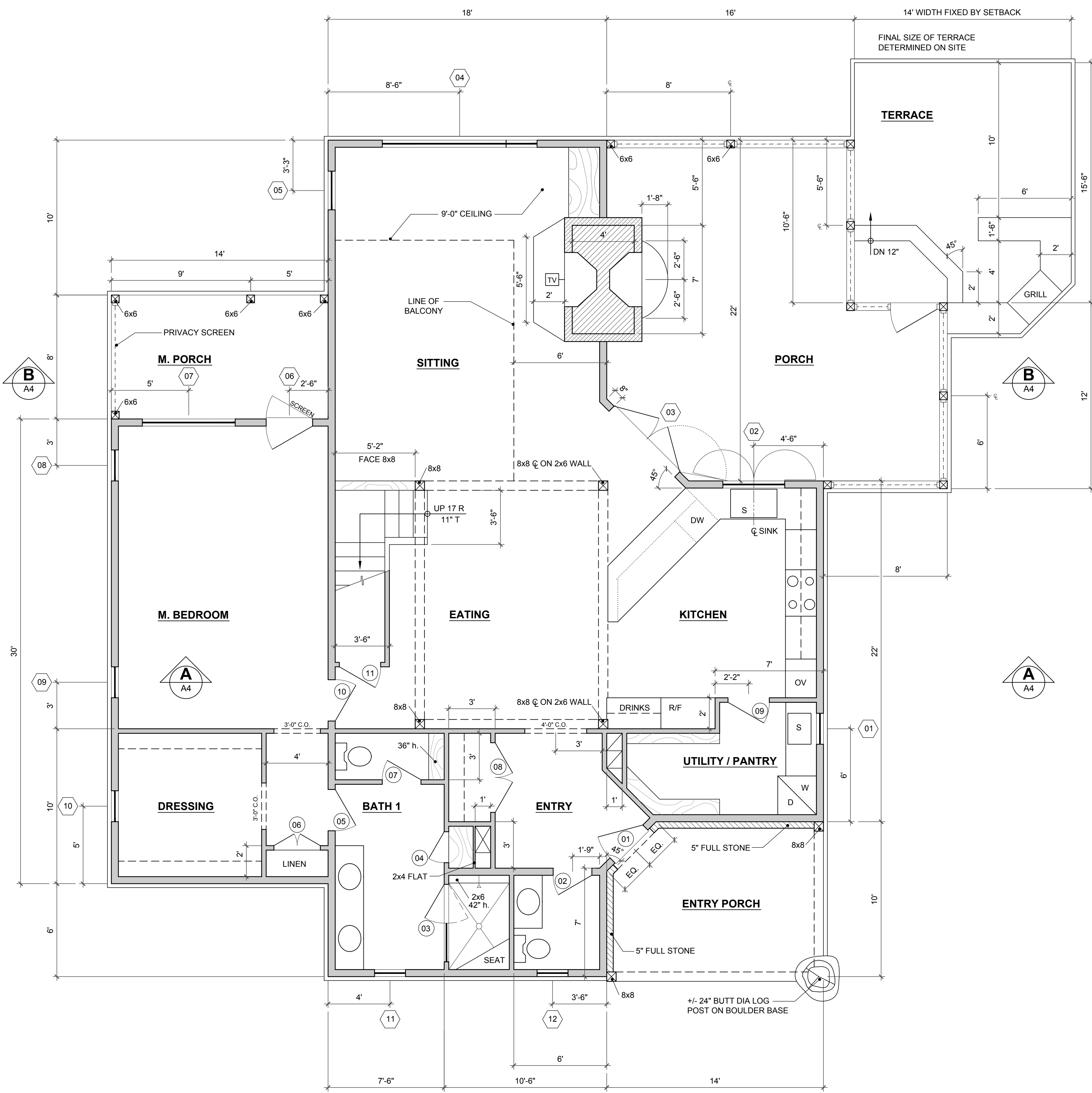
MAIN LEVEL FLOOR PLAN SCALE 1/4" = 1'-0"
