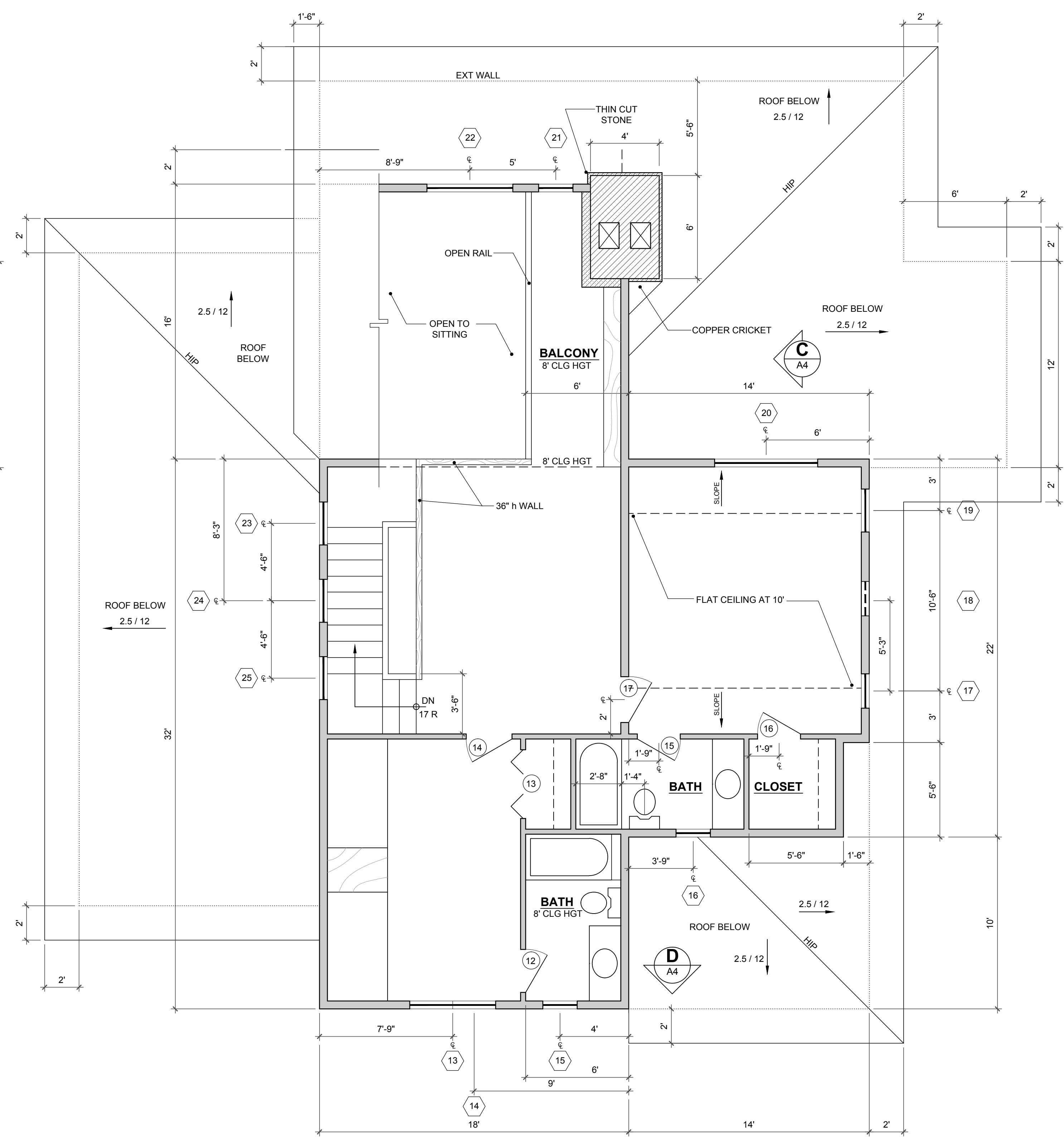
UPPER LEVEL FLOOR PLAN SCALE 1/4" = 1'-0"
